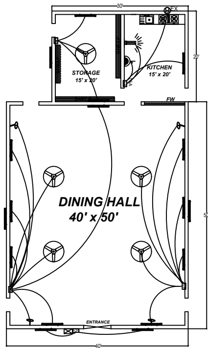
ELECTRICAL PLAN
